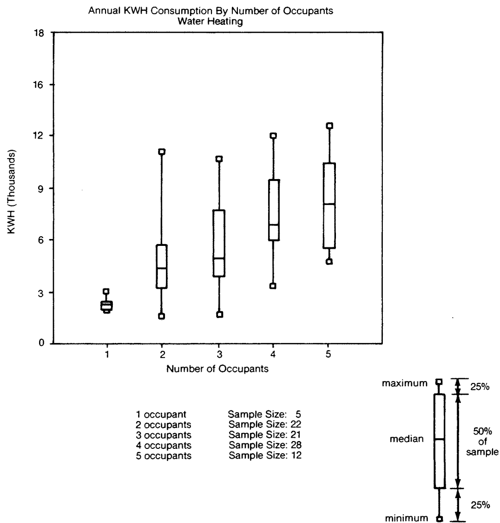
Figure K-2. Average Water Heat Consumption by Household Size
